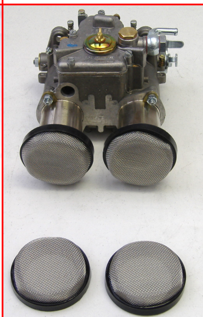
$35.00 99217.250 (Pair) Filter fits on air horn bell using patented lip lock technology with radiused entry for great signal and air flow. Three layer stainless steel filtering down to .009 with virtually no air flow restrictions
